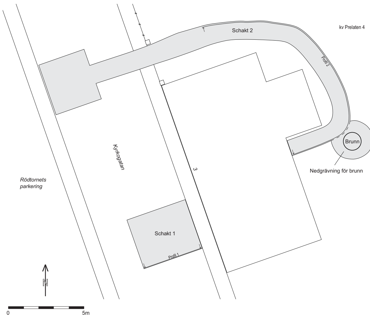
Figur 7. Schaktplan. Skala 1:150
